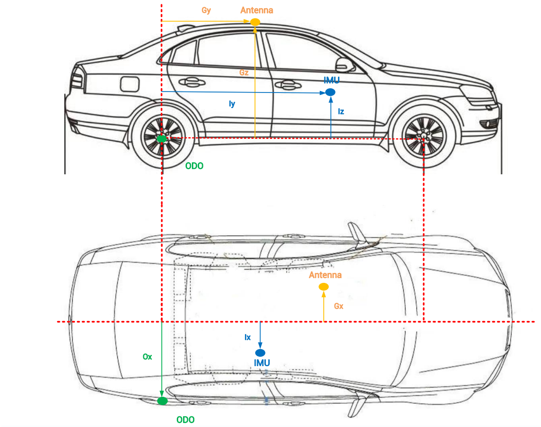
Figure 3-1 Lever Arm Configurations
