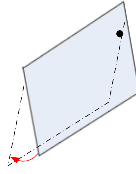
Rotate the module \beta deg around the Y axis (right-hand screw rule)
